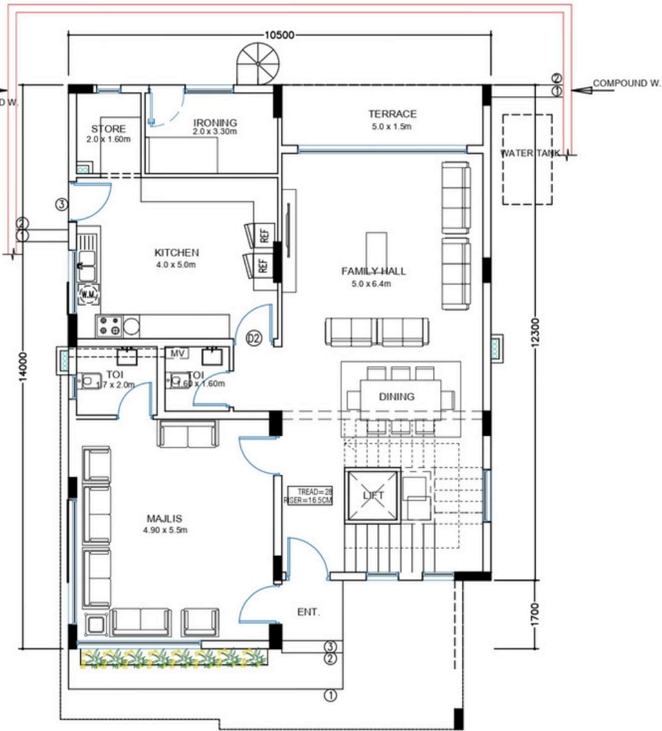
GROUND FLOOR PLAN SCALE 1:100 FLOOR AREA :1,510.91 sq ft
